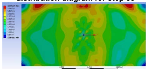
Figure 64 Equivalent stress (Von Mises) distribution diagram for step 60
