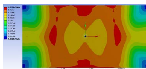
Figure 75 Equivalent stress (Von Mises) distribution diagram for step 71
