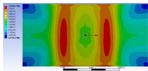
Figure 35 Equivalent stress (Von Mises) distribution diagram for step 31
