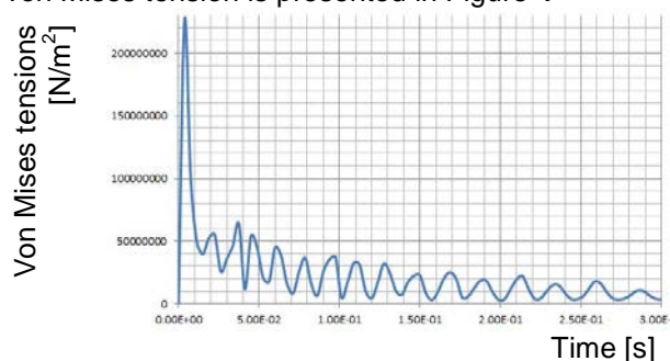
Figure 4 Time evolution of the maximum von Mises stress
