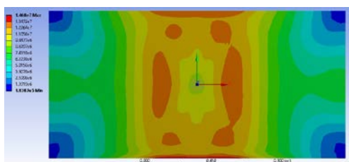
Figure 68 Equivalent stress (Von Mises) distribution diagram for step 64
