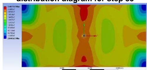
Figure 40 Equivalent stress (Von Mises) distribution diagram for step 36
