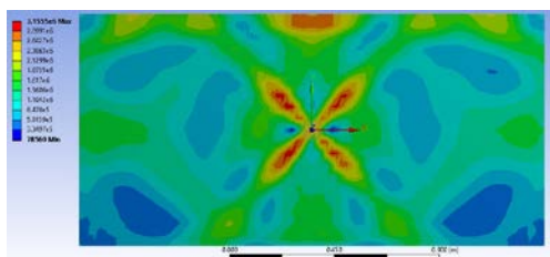
Figure 47 Equivalent stress (Von Mises) distribution diagram for step 43
