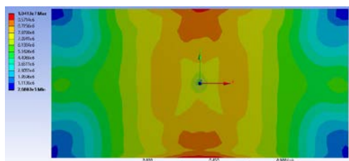
Figure 81 Equivalent stress (Von Mises) distribution diagram for step 77
