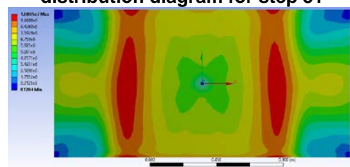
Figure 36 Equivalent stress (Von Mises) distribution diagram for step 32
