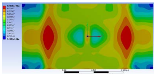
Figure 8 Equivalent stress (Von Mises) distribution diagram for step 4
