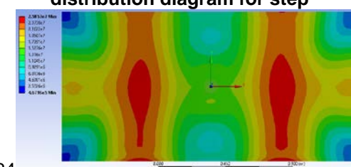
24 Figure 29 Equivalent stress (Von Mises) distribution diagram for step 25
