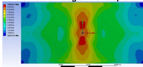
Figure 66 Equivalent stress (Von Mises) distribution diagram for step 62
