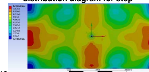
Figure 24 Equivalent stress (Von Mises) distribution diagram for step 20
