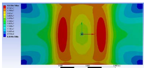
Figure 18 Equivalent stress (Von Mises) distribution diagram for step 14
