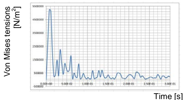
Figure 3 Time evolution of the minimum von Mises stress
