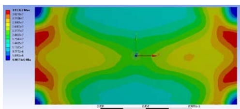
Figure 9 Equivalent stress (Von Mises) distribution diagram for step 5
