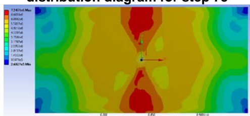
Figure 80 Equivalent stress (Von Mises) distribution diagram for step 76
