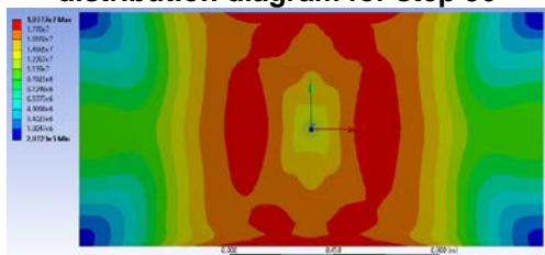
Figure 61 Equivalent stress (Von Mises) distribution diagram for step 57
