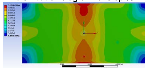
Figure 63 Equivalent stress (Von Mises) distribution diagram for step 59
