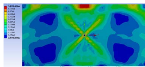
Figure 85 Equivalent stress (Von Mises) distribution diagram for step 81
