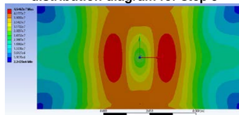
Figure 14 Equivalent stress (Von Mises) distribution diagram for step 10
