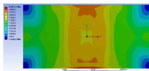
Figure 44 Equivalent stress (Von Mises) distribution diagram for step 40
