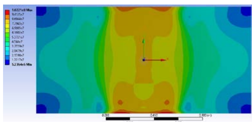
Figure 7 Equivalent stress (Von Mises) distribution diagram for step 3
