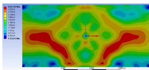
Figure 37 Equivalent stress (Von Mises) distribution diagram for step 33
