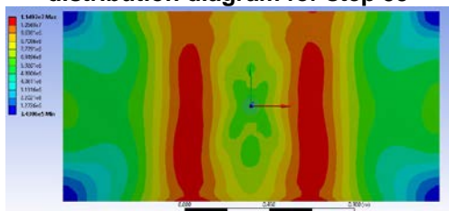
Figure 60 Equivalent stress (Von Mises) distribution diagram for step 56
