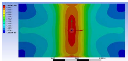
Figure 17 Equivalent stress (Von Mises) distribution diagram for step 13
