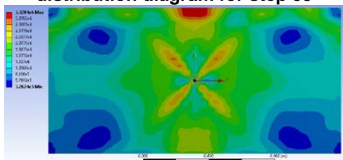
Figure 58 Equivalent stress (Von Mises) distribution diagram for step 54
