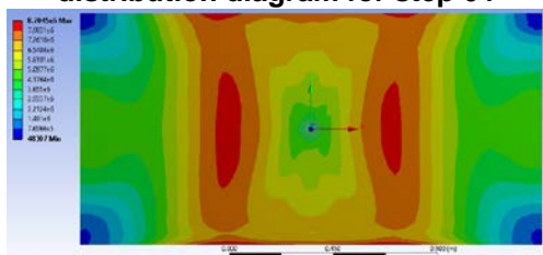
Figure 69 Equivalent stress (Von Mises) distribution diagram for step 65
