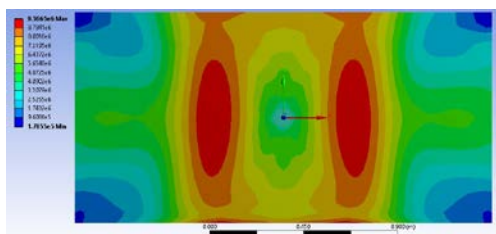
Figure 57 Equivalent stress (Von Mises) distribution diagram for step 53
