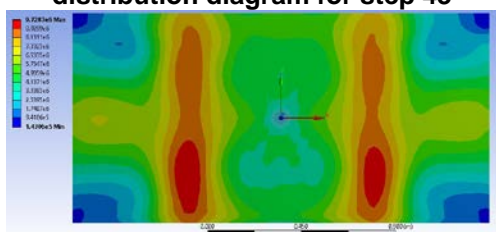
Figure 48 Equivalent stress (Von Mises) distribution diagram for step 44
