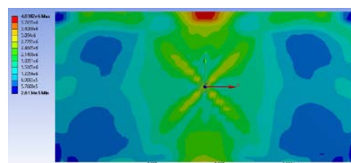
Figure 84 Equivalent stress (Von Mises) distribution diagram for step 80
