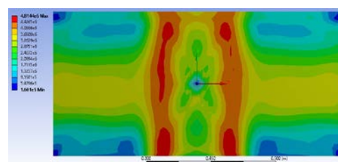
Figure 32 Equivalent stress (Von Mises) distribution diagram for step 28
