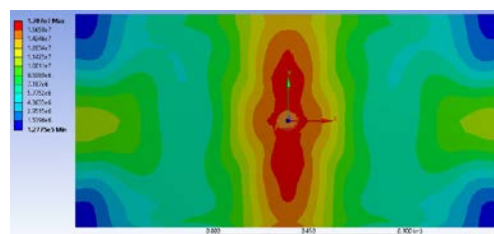
Figure 43 Equivalent stress (Von Mises) distribution diagram for step 39
