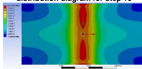
Figure 15 Equivalent stress (Von Mises) distribution diagram for step 11
