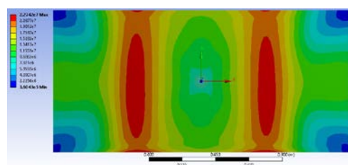
Figure 45 Equivalent stress (Von Mises) distribution diagram for step 41
