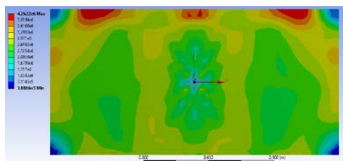
Figure 77 Equivalent stress (Von Mises) distribution diagram for step 73
