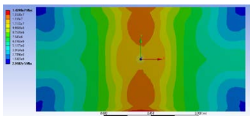
Figure 67 Equivalent stress (Von Mises) distribution diagram for step 63
