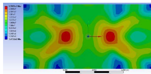
Figure 12 Equivalent stress (Von Mises) distribution diagram for step 8
