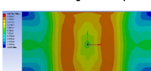
Figure 56 Equivalent stress (Von Mises) distribution diagram for step 52
