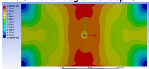
Figure 50 Equivalent stress (Von Mises) distribution diagram for step 46
