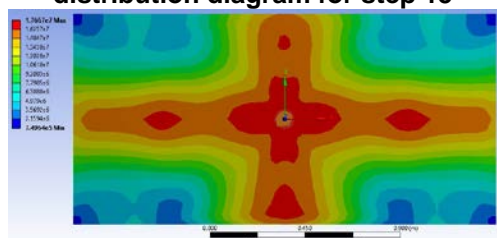
Figure 20 Equivalent stress (Von Mises) distribution diagram for step 16
