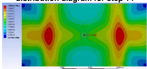
Figure 19 Equivalent stress (Von Mises) distribution diagram for step 15
