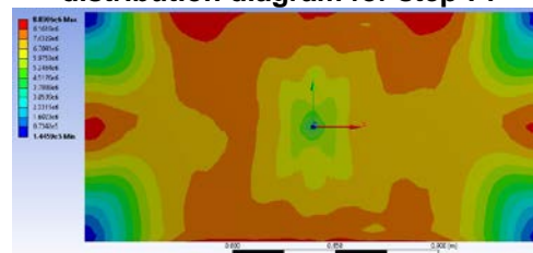
Figure 76 Equivalent stress (Von Mises) distribution diagram for step 72
