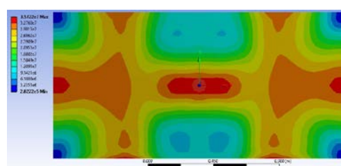
Figure 13 Equivalent stress (Von Mises) distribution diagram for step 9
