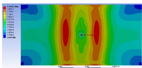
Figure 27 Equivalent stress (Von Mises) distribution diagram for step 23
