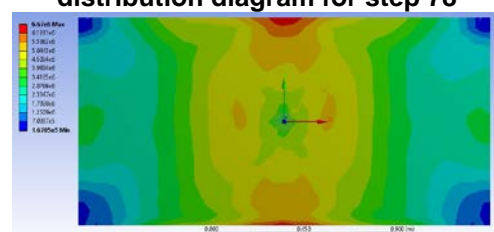
Figure 83 Equivalent stress (Von Mises) distribution diagram for step 79
