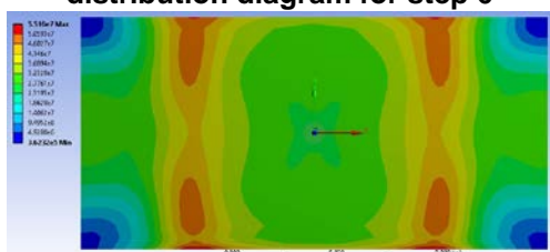
Figure 11 Equivalent stress (Von Mises) distribution diagram for step 7
