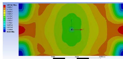
Figure 22 Equivalent stress (Von Mises) distribution diagram for step 18
