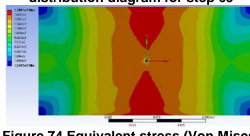
Figure 74 Equivalent stress (Von Mises) distribution diagram for step 70
