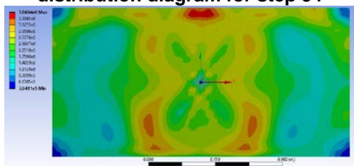
Figure 59 Equivalent stress (Von Mises) distribution diagram for step 55
