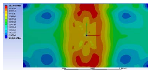
Figure 72 Equivalent stress (Von Mises) distribution diagram for step 68
