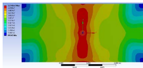
Figure 62 Equivalent stress (Von Mises) distribution diagram for step 58
