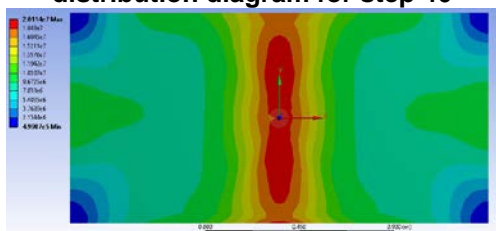
Figure 51 Equivalent stress (Von Mises) distribution diagram for step 47
