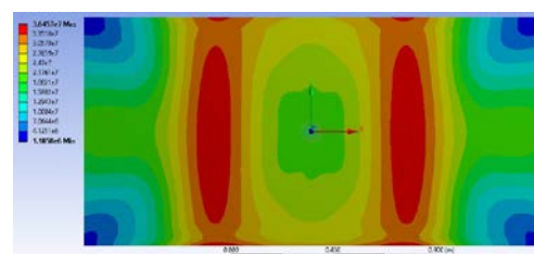
Figure 26 Equivalent stress (Von Mises) distribution diagram for step 22
