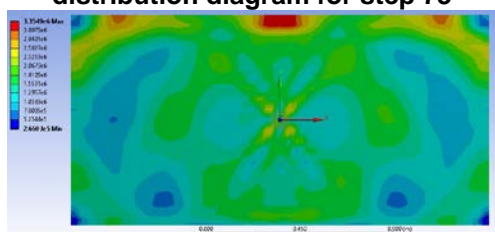
Figure 78 Equivalent stress (Von Mises) distribution diagram for step 74
