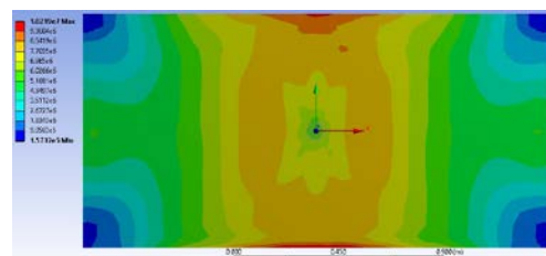
Figure 82 Equivalent stress (Von Mises) distribution diagram for step 78
