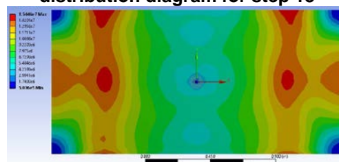
Figure 23 Equivalent stress (Von Mises) distribution diagram for step 19
