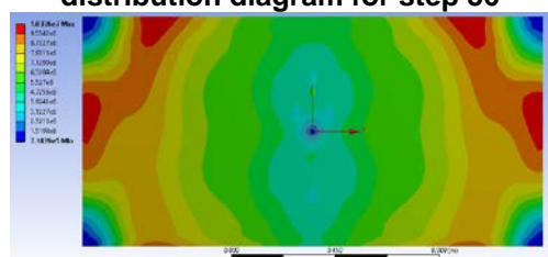
Figure 41 Equivalent stress (Von Mises) distribution diagram for step 37
