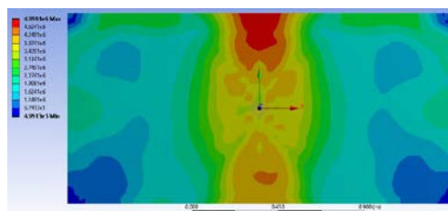
Figure 52 Equivalent stress (Von Mises) distribution diagram for step 48
